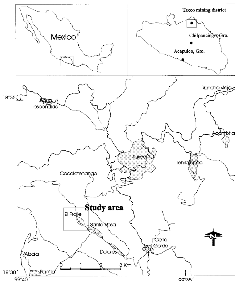
Figure 1. Study area.
